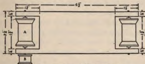
FIG. 162. — Top View of Wooden Frame.
